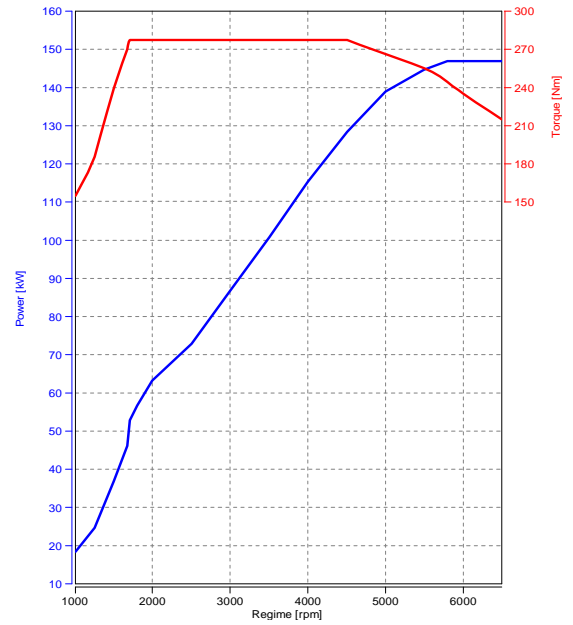
Performances curves
